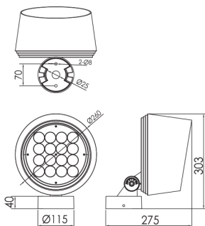
Surface Mount
