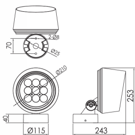
Surface Mount
