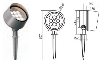
Stake Mount
