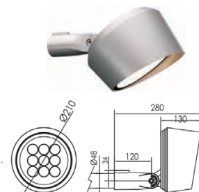
Pole Mount
