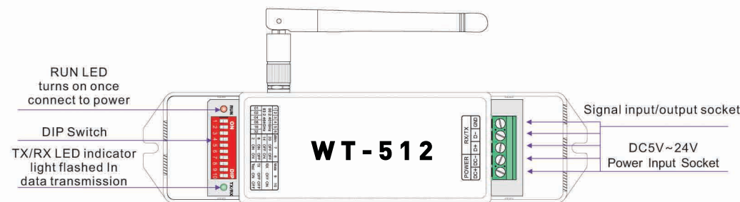
WT-512 wireless transceiver
